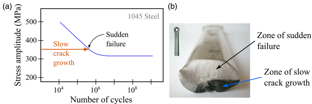
Fig. 1 Information on mechanical fatigue damage. (a) Mechanical fatigue damage in steel, according to Ref. 12. A chosen stress amplitude is applied and removed for a high number of cycles. During the first cycles, a small crack is initiated. The crack then grows slowly until the work piece breaks suddenly. (b) Photograph of an aluminum part that was subject to fatigue failure. 13
