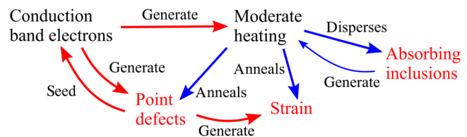
Fig. 3 Possible modifications of pre-existing fabrication defects during the incubation pulses.
