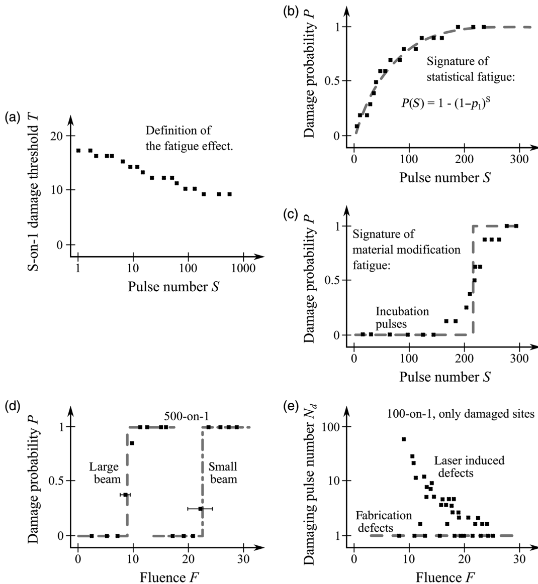
Fig. 2 Schematical summary of literature data. For references, please see the text. Dashed lines show expected dependencies for perfect lasers. Dots show typical data scattering for real lasers. (a) In case of a decreasing S-on-1 laser damage threshold T with increasing pulse number S (using otherwise identical measurement conditions), one speaks of a fatigue effect. (b) The damage probability P at constant fluence but varying pulse number S may show this shape that indicates statistical fatigue or the shape in (c), which indicates material modification fatigue. (d) For material modification fatigue, the obtained multi-pulse damage probability curves P(F) are deterministic (within the typical uncertainty of 10% in fluence). Smaller damage thresholds for larger test-beam sizes indicate an influence of self-focusing in the damage mechanism. (e) Shows all damaged sites in the fluence—shot number plane. Using the adapted beam size, one can observe “immediate” damage induced by fabrication defects as well as fatigue damage occurring for higher pulse numbers.
