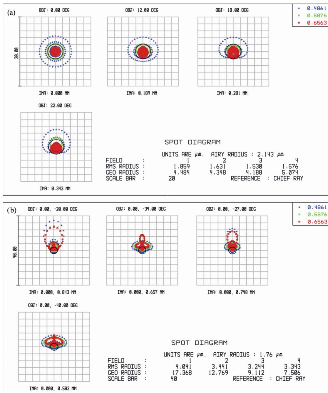
Fig. 6 Image surface spot diagram for (a) forward-view optics and (b) radial-view optics. The black circle is the simulated Airy Disk radius. The colors correspond to the wavelength legend at the top right of this figure; all units are in micrometers. RMS radius is the root mean square spot size, and GEO radius is the distance from the centroid to the furthest ray intersection with the imaging surface. IMA describes the location of the centroid on the imaging surface. OBJ describes the location of the field points in terms of field angles. The forward optics has smaller spot sizes than the sidewall optics.
