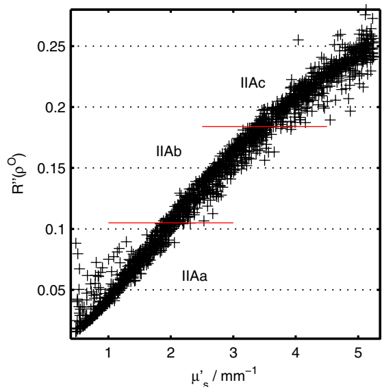
Fig. 4 Correlation between the second derivative R''(\rho^0) and the reduced scattering coefficient \mu'_s for all SRR curves of group IIA. The radial distance \rho^0 is the position where the SRR curve decreased 0.7 orders of magnitude relative to the reflectance value at \rho = 1 \text{ mm} .
