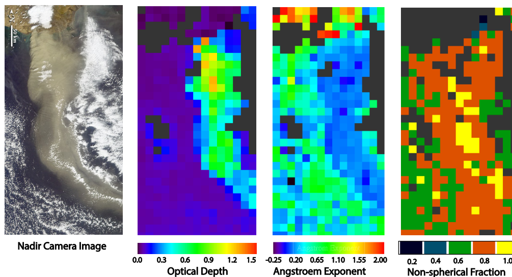
Fig. 2 An example of MISR air mass mapping applied to the Eyjafjalljökull plume on April 19, 2010. 24
