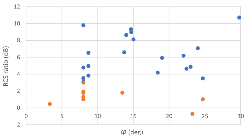
Fig. 8 Post- to pre-flood RCS ratio versus \phi for flooded urban DS pixels for Fishlake November 14, 2019 flooding (VV polarization). High RCS ratios (blue) are above the 3 dB threshold, orange ratios are below.
