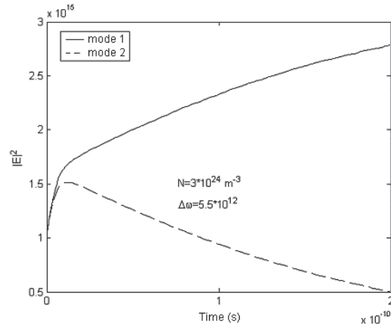
Fig. 2. Field intensities versus time for \Delta\omega = 5.5 \cdot 10^{-12}
