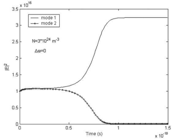
Fig. 1. Field intensities versus time for \Delta\omega = 0
