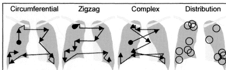
Figure 6 Three scanpath patterns that produce the same fixation distribution
