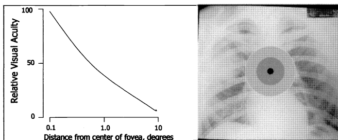
Figure 3. The relative visual acuity and the relative size of the associated field of view
