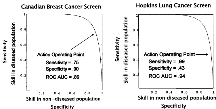
Figure 1. DOC curves for breast and lung cancer screening by projection images
