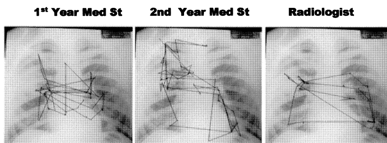
Figure 5. The scanpath of a first year medical student, a second year medical student and a radiologist looking at an image of a projection chest with two infiltrates.
