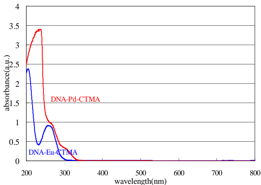
Fig. 3 UV-Vis spectra of DNA-CTMA-metal complexes in ethanol solutions
