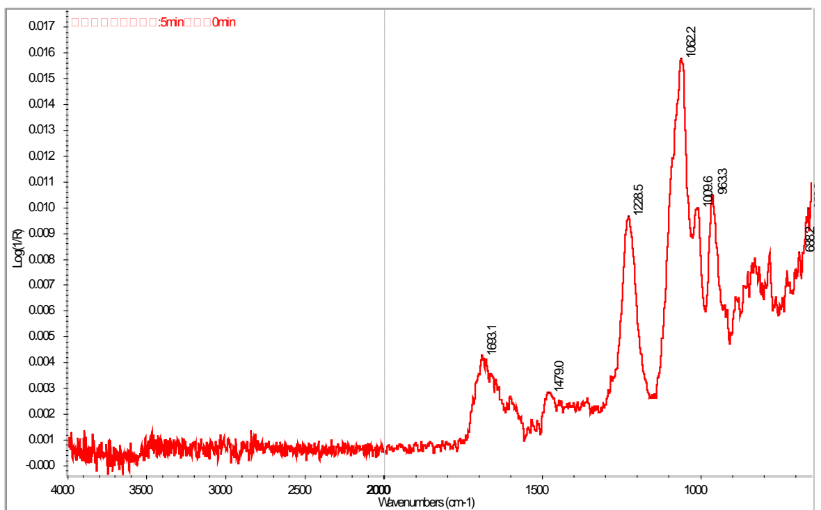
Fig.4 Differential infrared spectrum between non-irradiated and irradiated
