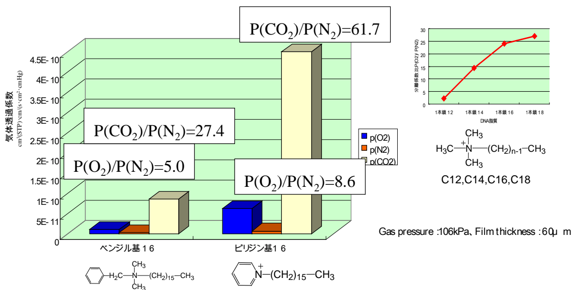
Fig. 10 Gas permeation data of various DNA films
