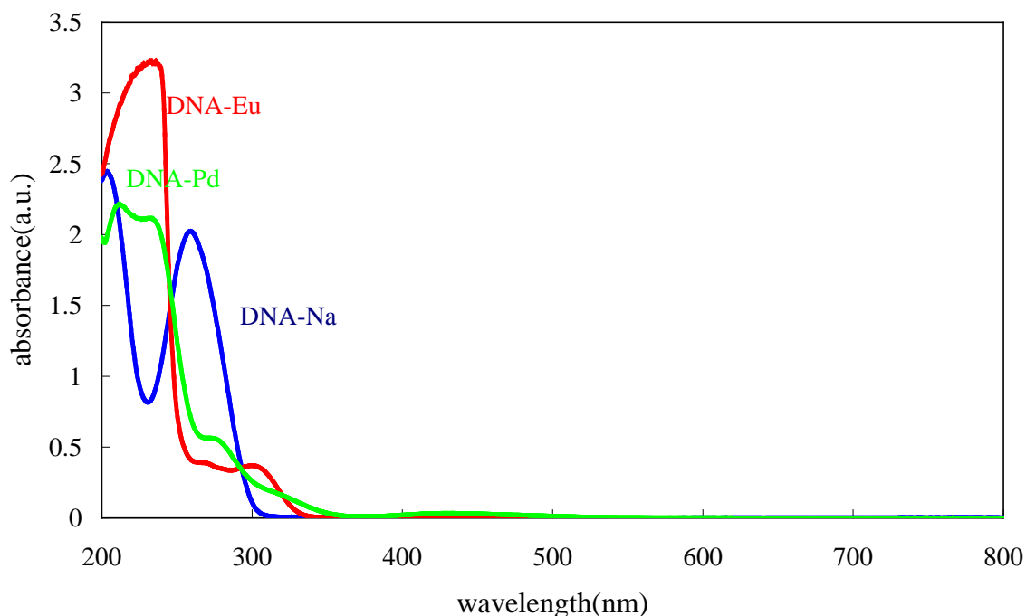
Fig. 2 UV-Vis spectra of aqueous solutions of DNA-metal complexes
