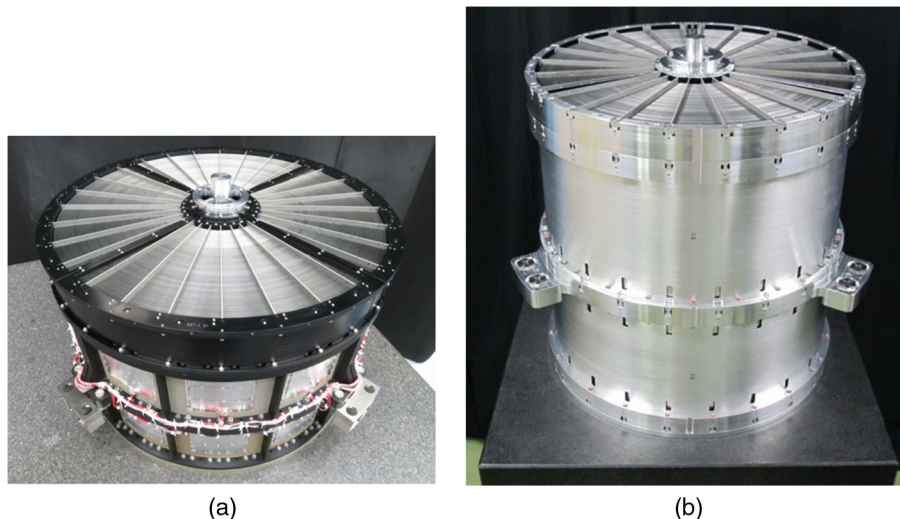
Fig. 4 Photographs of flight models of (a) Soft X-ray Telescope, SXT-S, and (b) Hard X-ray Telescope, HXT-1.
