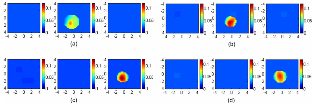
Fig. 7 Images of an excised mouse tumor reconstructed from different boundary conditions. The left column [(a) and (c)] was obtained using the absorbing boundary; the right column [(b) and (d)] using the aluminum cover. In (a) and (b), the tumor center was located at 1.0-cm depth. The reconstructed maximums were 0.088 and 0.122 \text{cm}^{-1} , respectively. In (c) and (d), the tumor center was located at 1.6-cm depth. The reconstructed maximums were 0.137 and 0.101 \text{cm}^{-1} , respectively.
