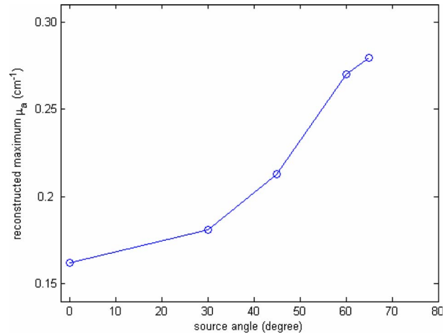
Fig. 11 The reconstructed maximum \mu_a when the source has different tilted angle. The background optical properties of the medium were \mu_a=0.03 \text{ cm}^{-1} and \mu'_s=6.0 \text{ cm}^{-1} . The target was located at the center (0, 0, 0.7 cm) with radius 0.5 cm and \mu_a=0.3 \text{ cm}^{-1} and \mu'_s=6.0 \text{ cm}^{-1} .
