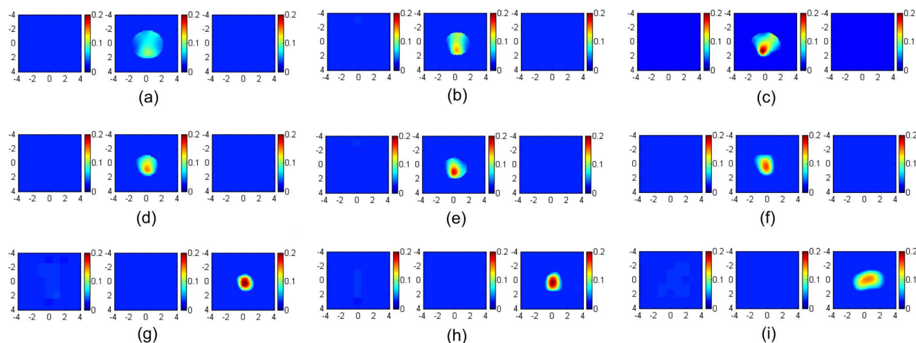
Fig. 5 Images of the high-contrast absorber reconstructed from different boundary conditions. The left column was obtained using the absorption boundary; the middle column was obtained using the absorption boundary with one angled source; the right column was obtained using the partial reflection boundary. In (a), (b), and (c), the target center was located at 0.7-cm depth. The first slice is the spatial x - y image of 8\text{ cm} \times 8\text{ cm} obtained at 0.2-cm depth, and the second and third cross-sections slice at 0.7- and 1.2-cm depths. In (d), (e), and (f), the target center was located at 1.0-cm depth. The first slice is obtained at 0.5 cm and the second and third at 1.0- and 1.5-cm depths. In (g), (h), and (i), the target center was located at 1.5-cm depth. The reconstructed maximum and mean values were shown in Table 1.
