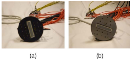
Fig. 1 Photograph of the new probe that incorporates an absorption boundary with an angled source (a) or a partial reflection boundary using an aluminum cover (b). The ultrasound probe was located at the center and the optical source and detector fibers were distributed at the periphery of the ultrasound probe.
