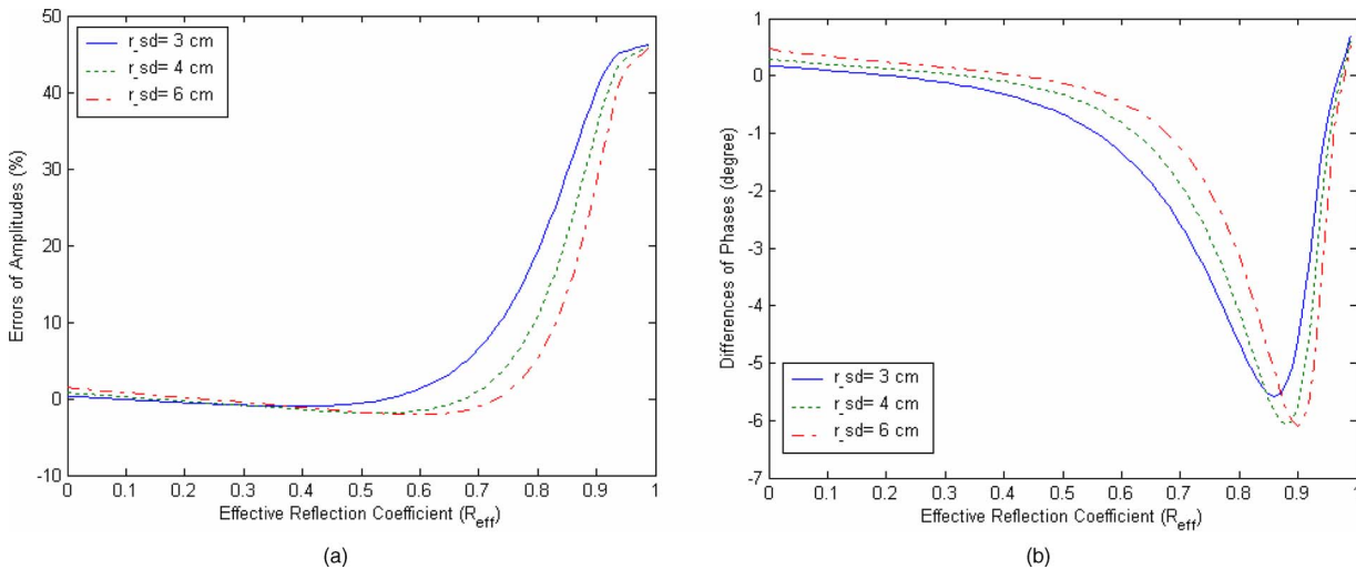
Fig. 4 Errors between two boundary conditions as a function of effective reflection coefficient. Three typical source-detector distances of 3, 4, and 6 cm were shown in figures. (a) Relative errors of amplitude. (b) Phase errors.
