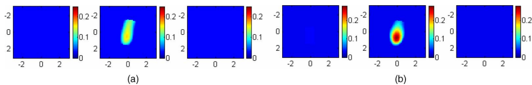
Fig. 8 The reconstructed image for a simulated target using the black probe with normal-incident sources (a) and the angled probe (b). The background optical properties of the medium were \mu_a=0.03 \text{ cm}^{-1} and \mu'_s=6.0 \text{ cm}^{-1} . The target was located at the center (0, 0, 0.7 cm) with radius 0.5 cm and \mu_a=0.3 \text{ cm}^{-1} and \mu'_s=6.0 \text{ cm}^{-1} . For both images, the first slice is the spatial x - y image of 6 \text{cm} \times 6 \text{ cm} obtained at 0.2 cm, and the second slice is at the depth of 0.7 cm with 0.5-cm spacing between slices. In (a), the maximum reconstructed value was \mu_a=0.162 \text{ cm}^{-1} (54% of the true value), and in (b), the maximum \mu_a=0.27 \text{ cm}^{-1} (90%).
