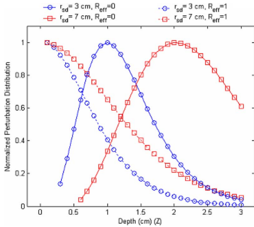
Fig. 3 Perturbation distribution as a function of the target depth for an absorption boundary ( R_{eff}=0 ) and reflection boundary ( R_{eff}=1 ). Two typical source-detector distances of 3 and 7 cm were selected.
