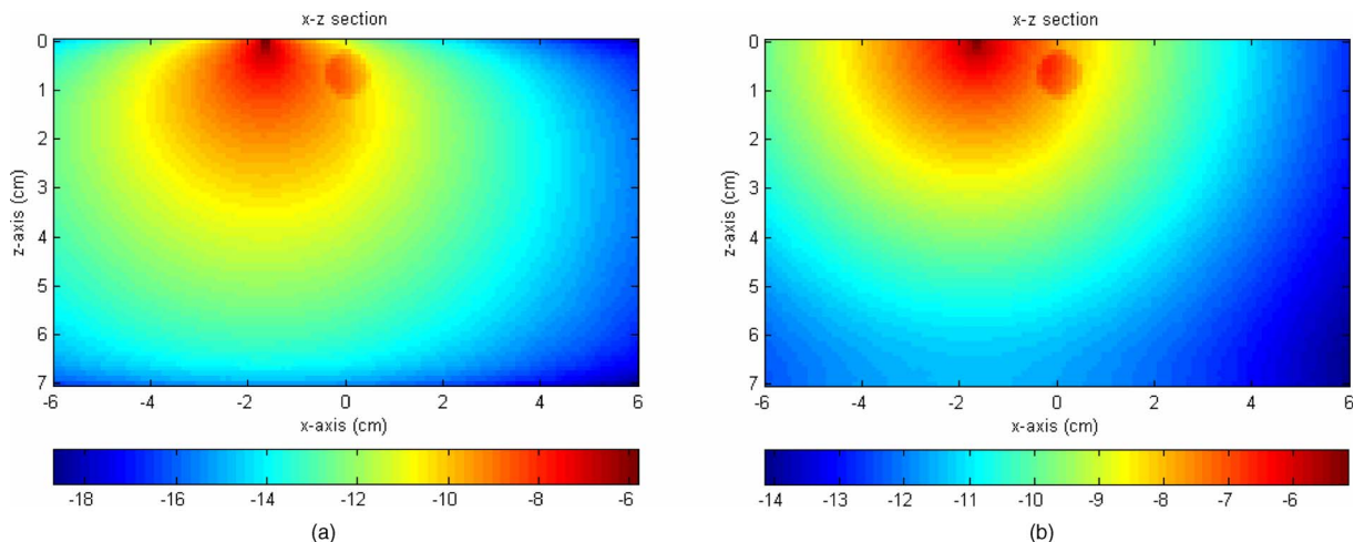
Fig. 2 Logarithmic scale display of absorption distributions inside the medium computed using an absorption boundary (a) and a reflection boundary (b). The medium has dimensions of 12\times 12\times 7\text{ cm}^3 . The figure was displayed as x-z projection; x axis is the lateral dimension and z is the depth. The medium background optical properties were \mu_a=0.03\text{ cm}^{-1} and \mu'_s=6.0\text{ cm}^{-1} ; the target optical properties were \mu_a=0.3\text{ cm}^{-1} and \mu'_s=6.0\text{ cm}^{-1} . The target was a 0.5-cm radius sphere located at (0, 0, 0.7 cm), and the source was located at (-1.7 cm, 0, 0).
