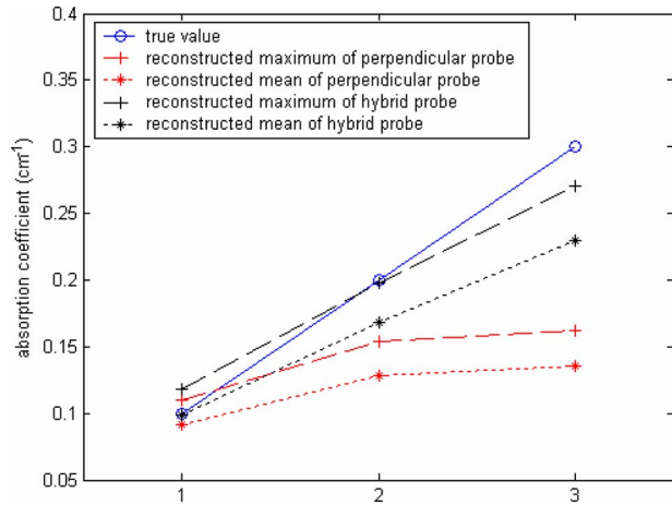
Fig. 9 Reconstruction results for a 1-cm diameter spherical target at (0, 0, 0.7 cm) from the probe with all normal-incident sources and the angled probe with normal-incident sources and one angled source.
