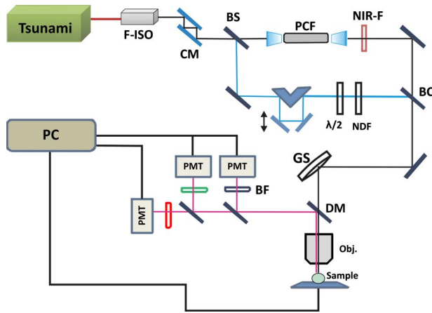
Fig. 1 Schematic of the inhouse-built nonlinear optical laser-scanning microscope with the Stokes pulses being generated in PCF, which is synchronously pumped by the same Ti:sapphire laser that provides the pump pulse. F-ISO: Faraday isolator; CM: chiral laser mirrors; BS: beamsplitter; NIR-F: near-IR filter; BC: beam combiner; GS: galvo scanner; DM: dichroic mirror; OBJ: objective lens; BF: bandpass filter; NDF: neutral density filter; and \lambda/2 : half waveplate.
