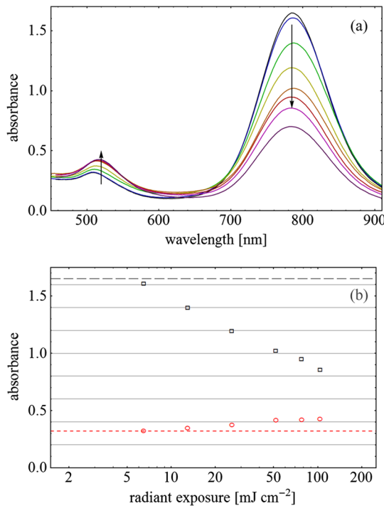
Fig. 10 (a) UV/VIS spectra of nanorod suspension after irradiation with five pulses at 785 nm: black—non-irradiated, blue-6.5 \text{mJ cm}^{-2} , green-13 \text{mJ cm}^{-2} , yellow-26 \text{mJ cm}^{-2} , orange-52 \text{mJ cm}^{-2} , red-78 \text{mJ cm}^{-2} , magenta-104 \text{mJ cm}^{-2} . The arrows indicate change of absorption due to increase of the radiant exposure. (b) Change of peak absorption of the TSPR (red circles) and LSPR band (black squares) with radiant exposure. The black and the red dashed lines indicate the absorbance of nanorods that were not irradiated.
